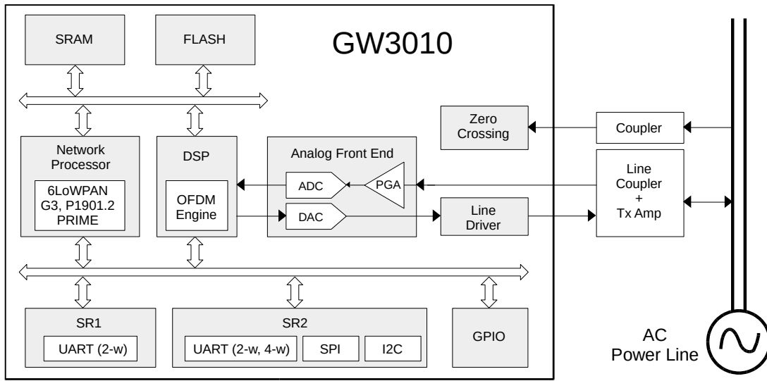
Figure 1 Functional Block Diagram of the GW3010
